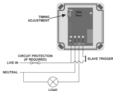
Diagram 1 Standard Wiring
